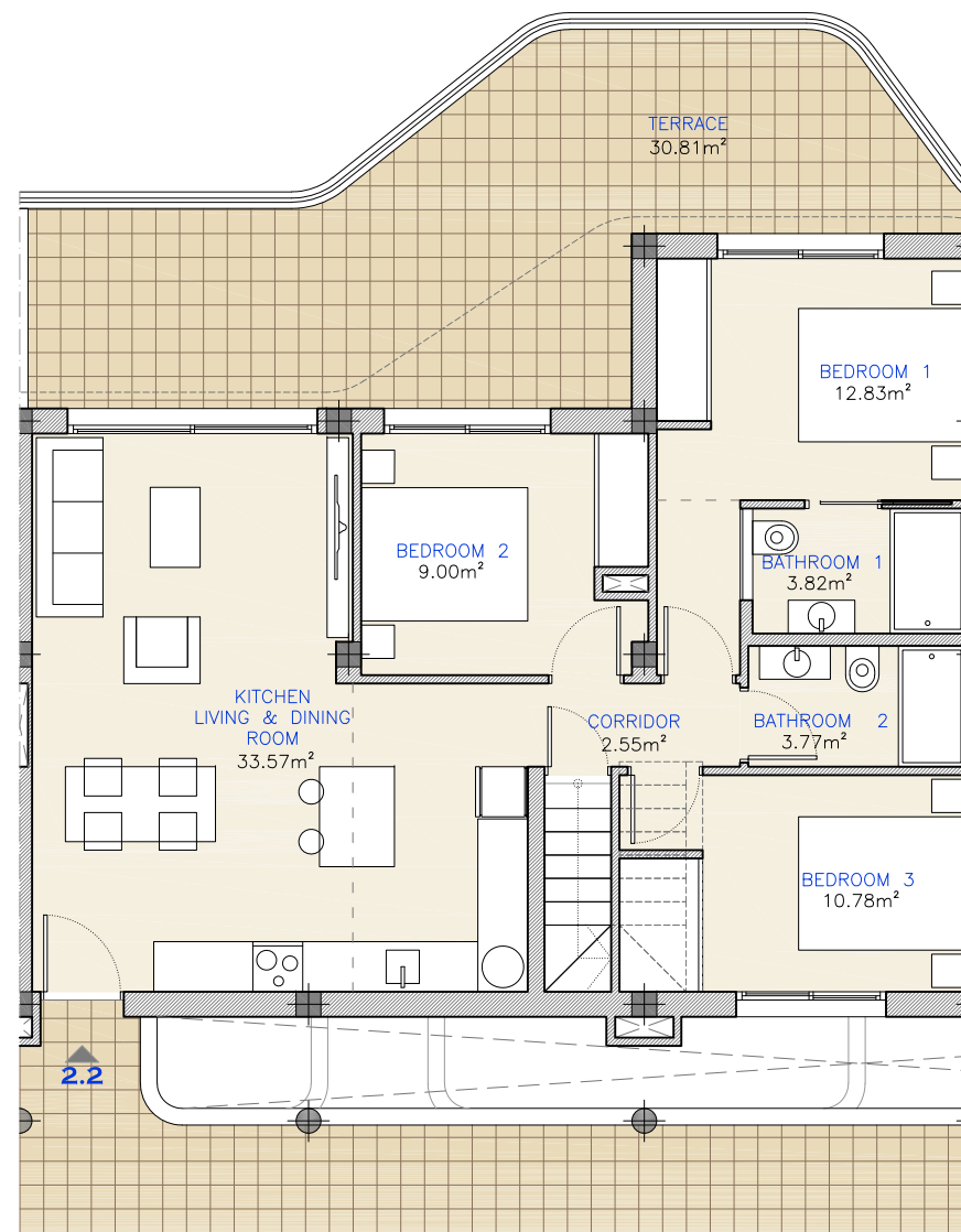
MAIN FLOOR
