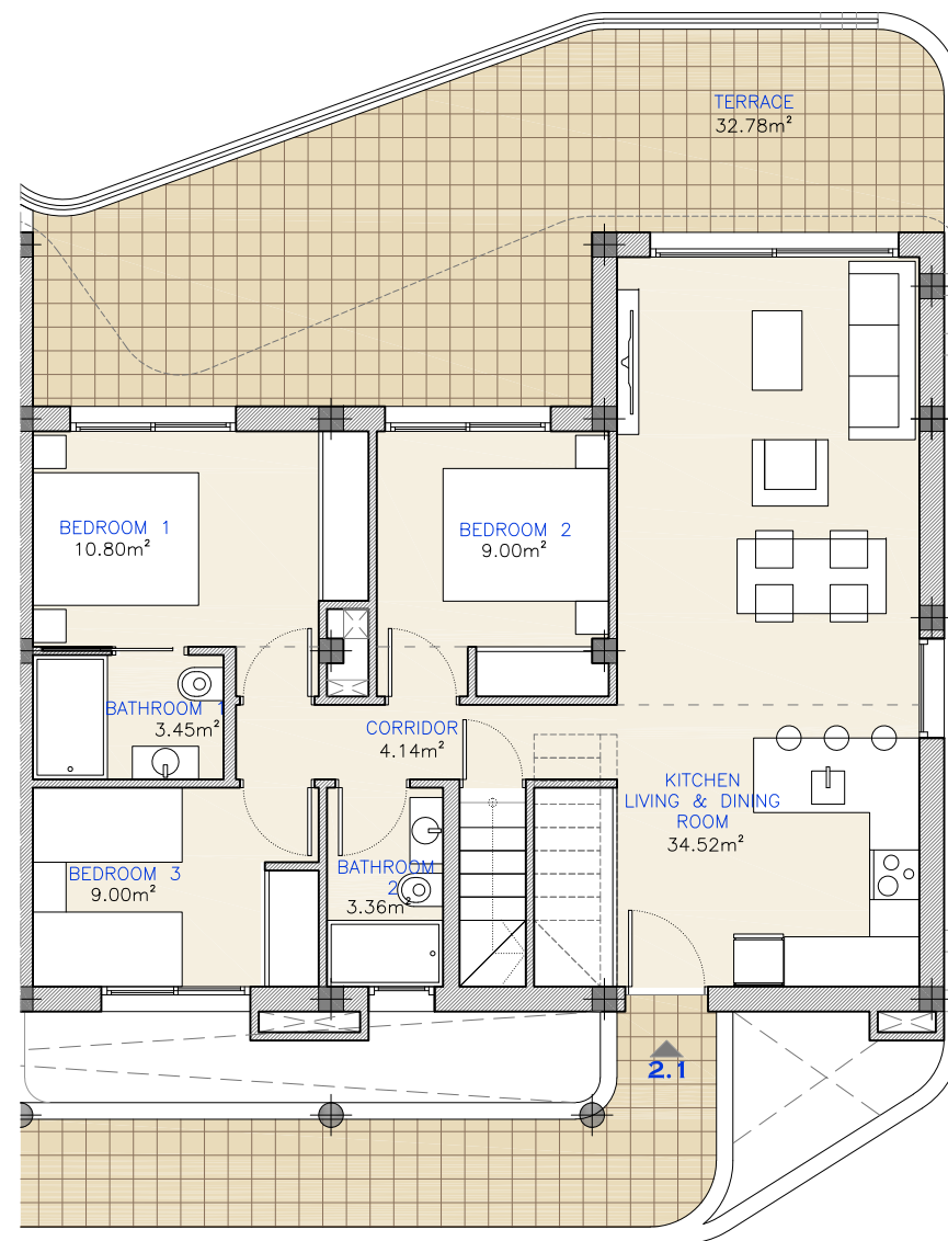
MAIN FLOOR
